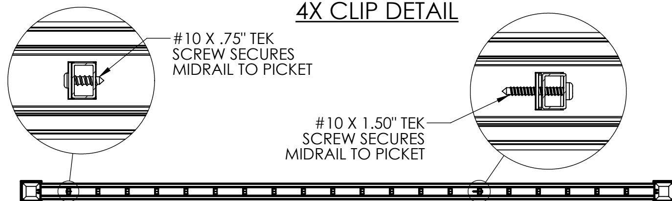
SECTION B-B
