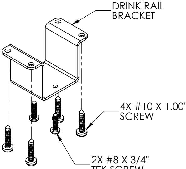
DRINK RAIL BRACKET DETAIL
