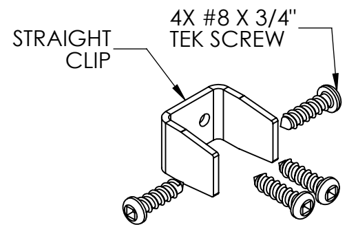
8X CLIP DETAIL
