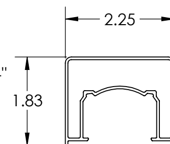
ALTA TOP RAIL IS AN ALTERNATIVE OPTION WITH A 42.04" OVERALL HEIGHT
