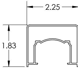
ALTA TOP RAIL IS AN ALTERNATIVE OPTION WITH A 42.05" OVERALL HEIGHT
