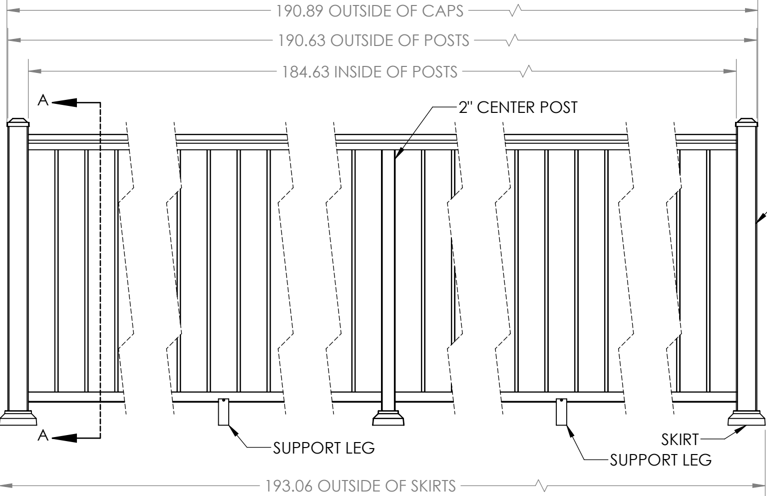
VICTORIAN TOP RAIL
