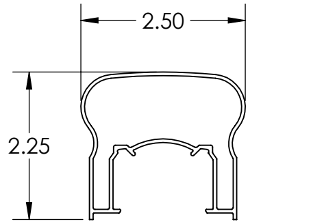
VICTORIAN TOP RAIL
